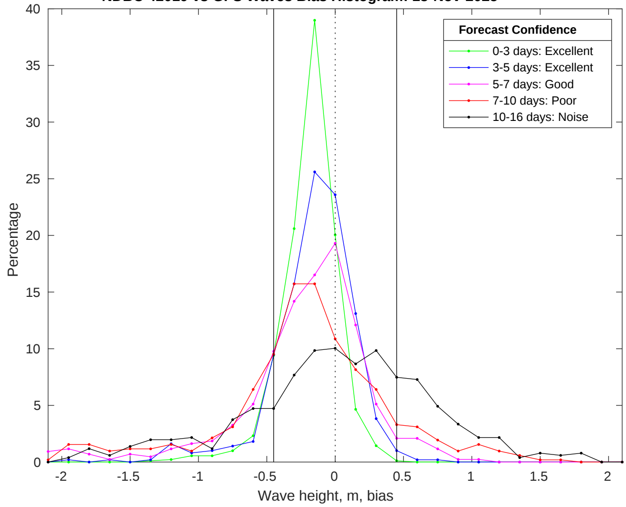
NDBC 42019 vs GFS Waves Bias Histogram: 13-Nov-2025
