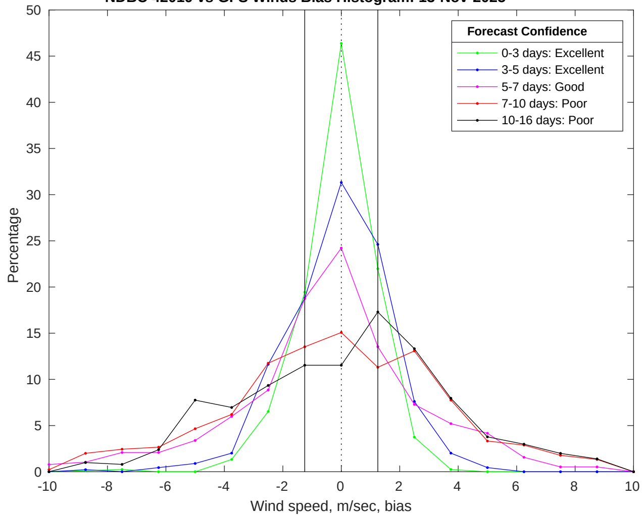
NDBC 42019 vs GFS Winds Bias Histogram: 13-Nov-2025
