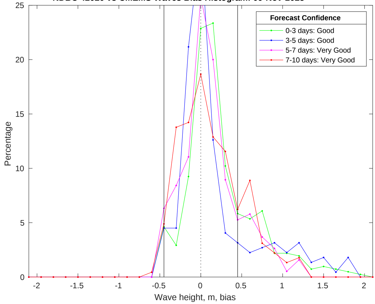
NDBC 42020 vs CMEMS Waves Bias Histogram: 09-Nov-2025
