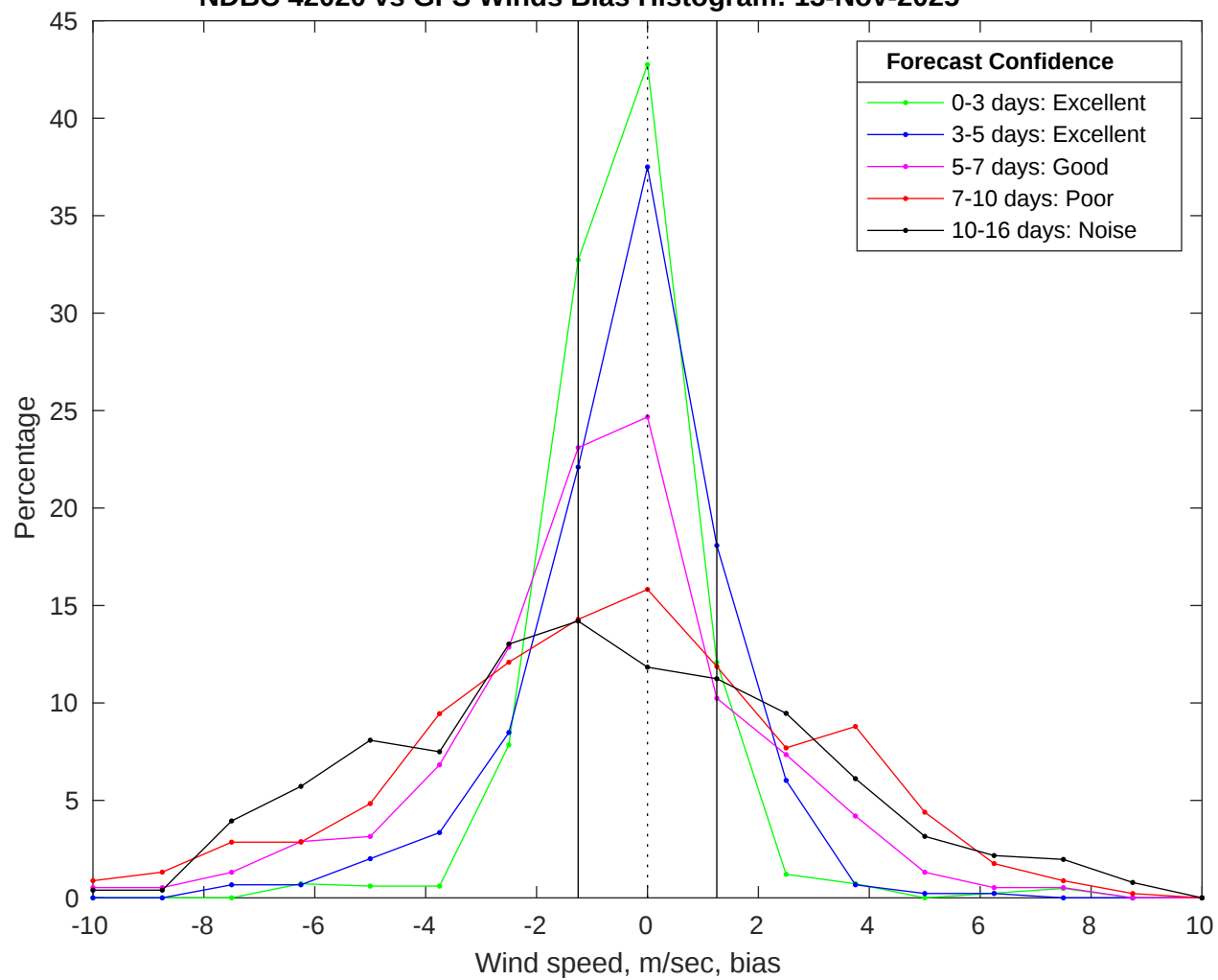
NDBC 42020 vs GFS Winds Bias Histogram: 13-Nov-2025
