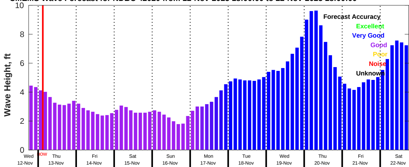
CMEMS Wave Forecast for NDBC 42020 from 12-Nov-2025 18:00:00 to 22-Nov-2025 18:00:00
