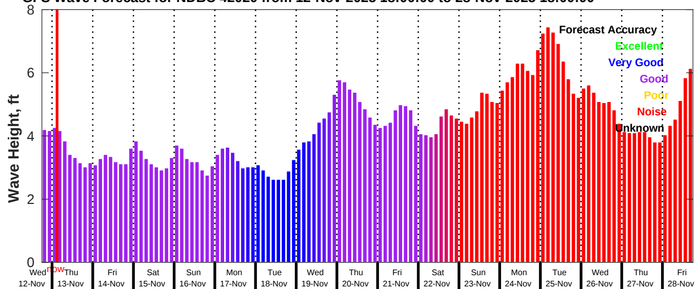
GFS Wave Forecast for NDBC 42020 from 12-Nov-2025 18:00:00 to 28-Nov-2025 18:00:00
