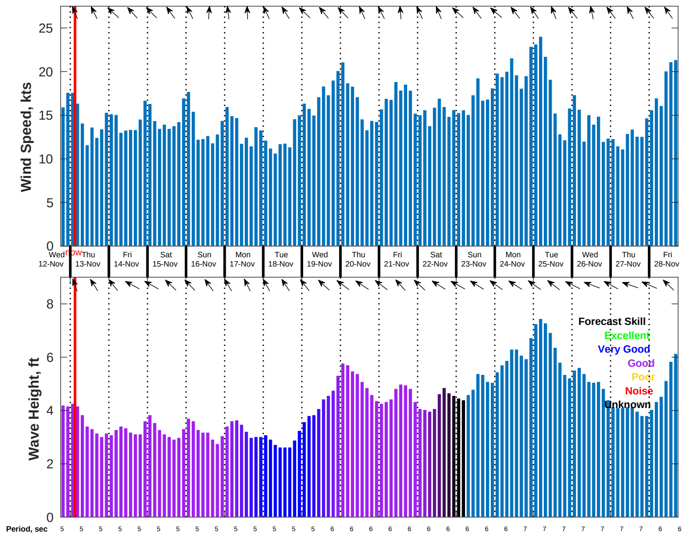
Wind & Wave Forecast for NDBC 42020 from 12-Nov-2025 18:00:00 to 28-Nov-2025 18:00:00
