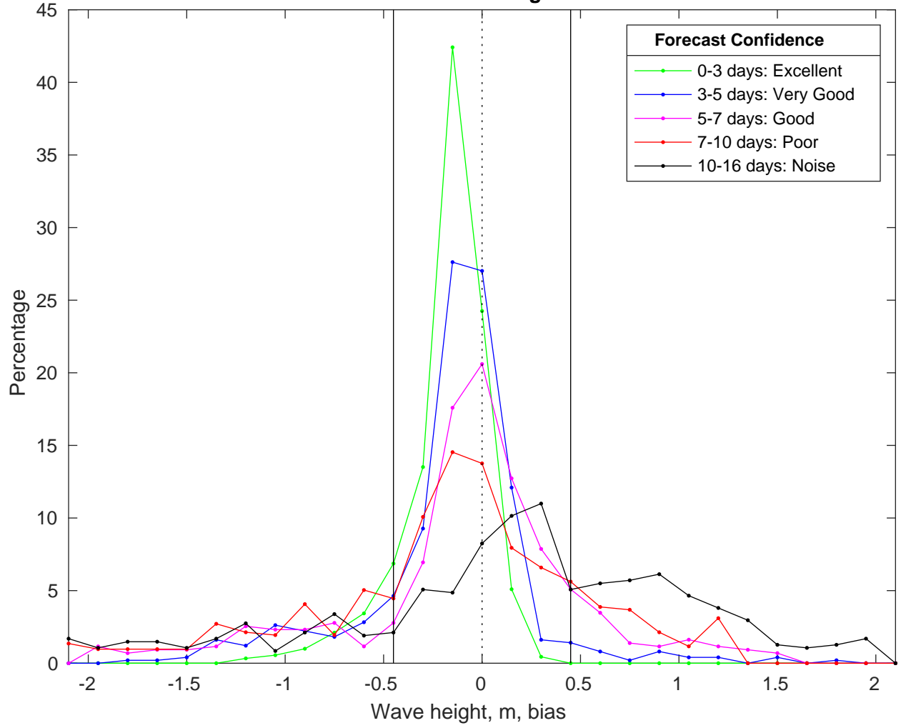
NDBC 42036 vs GFS Waves Bias Histogram: 13-Nov-2025
