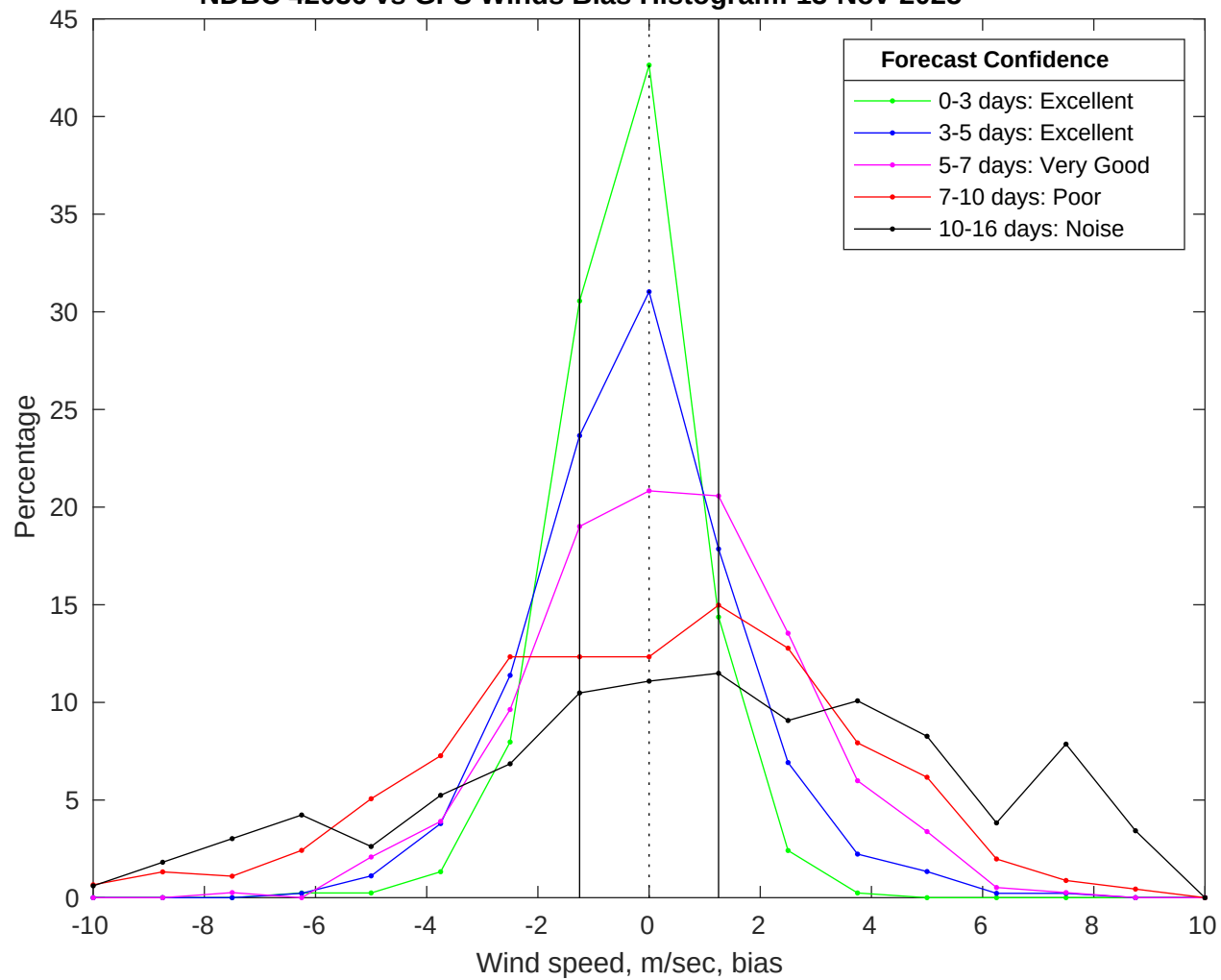
NDBC 42036 vs GFS Winds Bias Histogram: 13-Nov-2025
