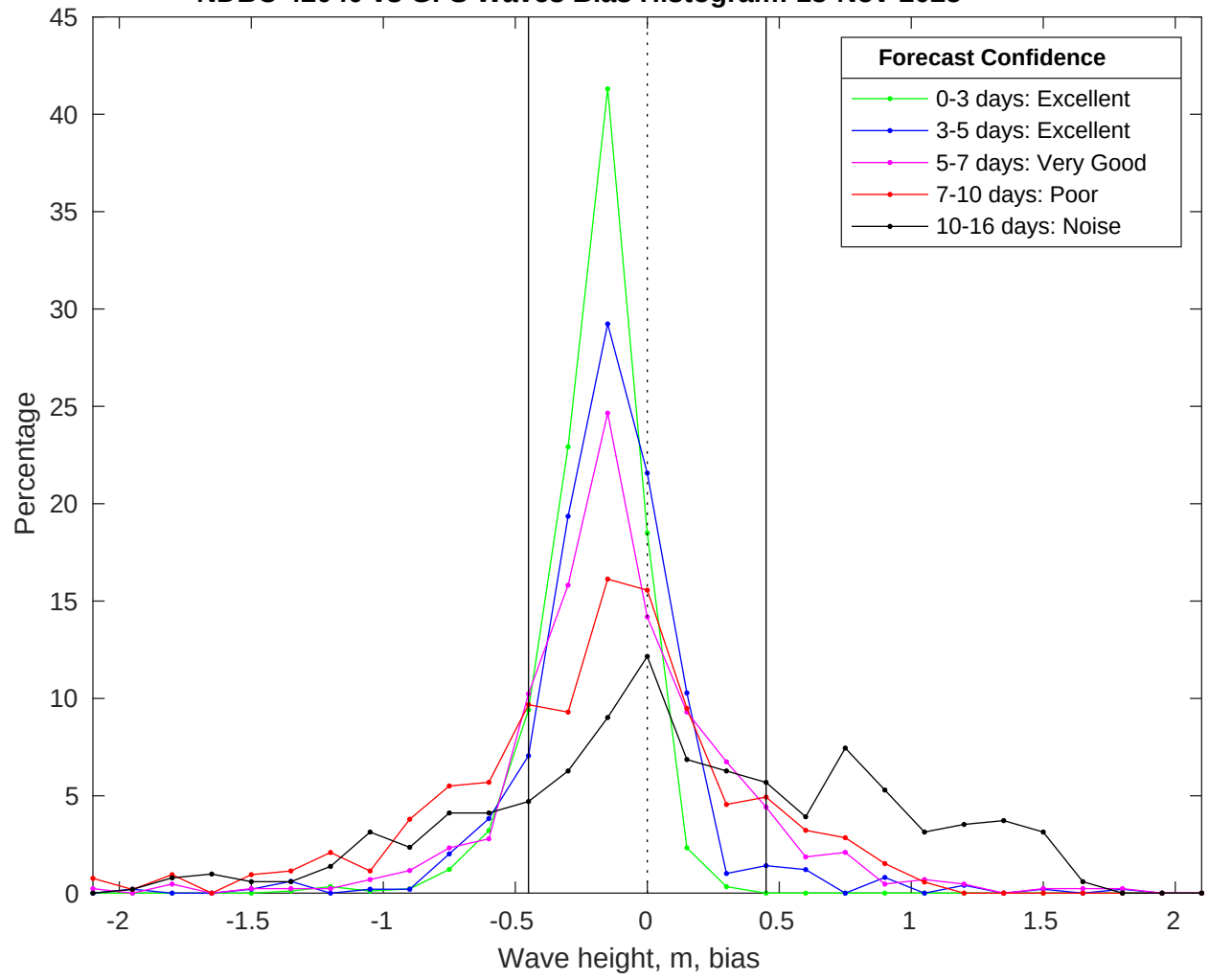
NDBC 42040 vs GFS Waves Bias Histogram: 13-Nov-2025
