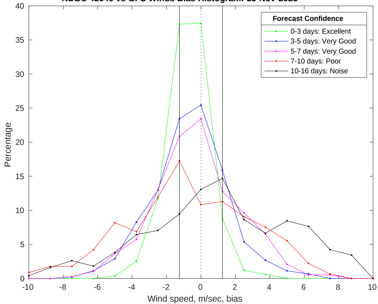
NDBC 42040 vs GFS Winds Bias Histogram: 13-Nov-2025
