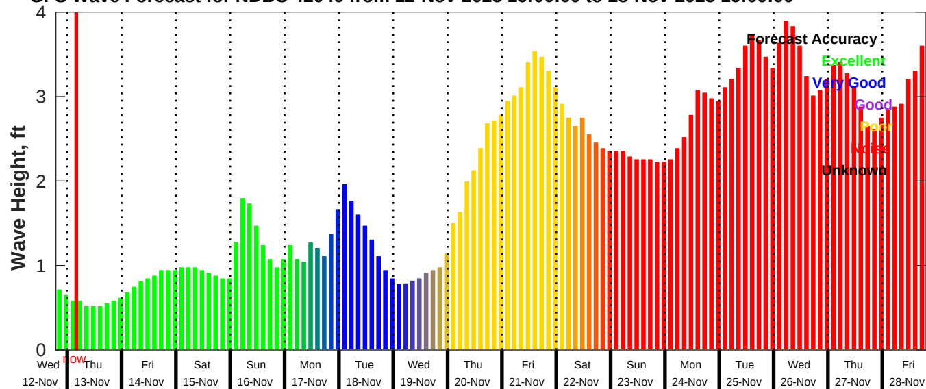
GFS Wave Forecast for NDBC 42040 from 12-Nov-2025 19:00:00 to 28-Nov-2025 19:00:00
