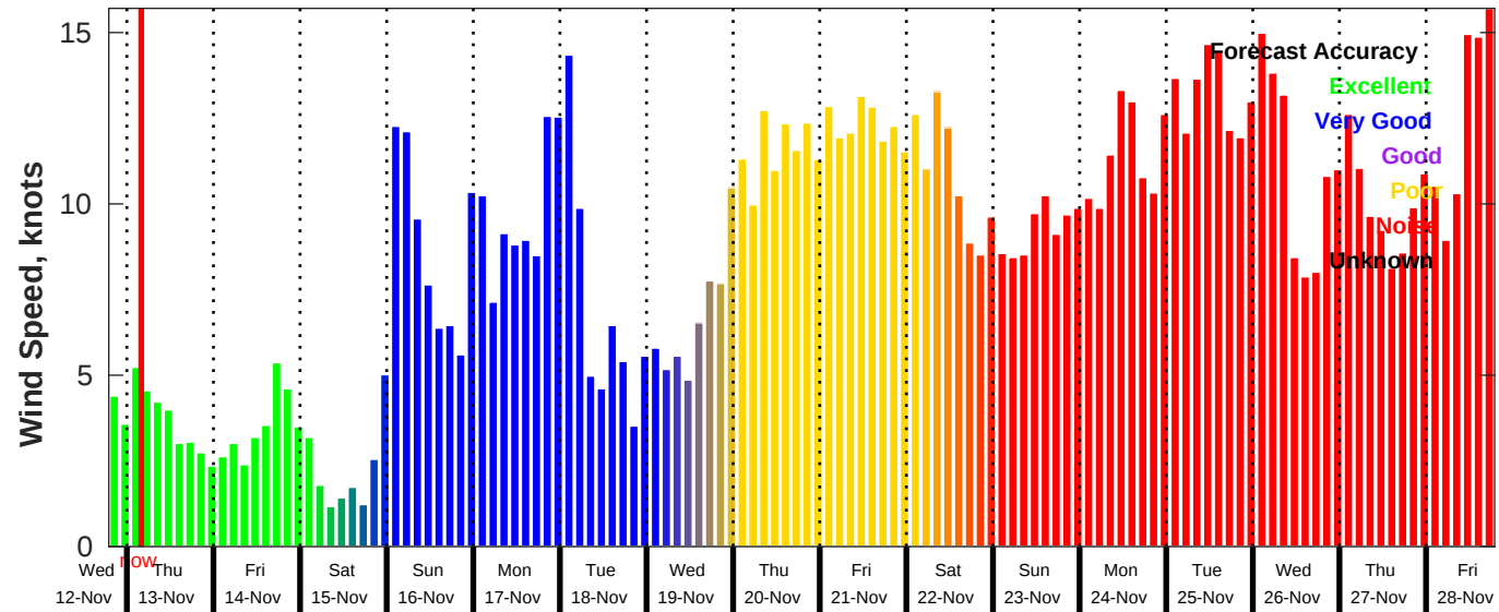
GFS Wind Speed Forecast for NDBC 42040 from 12-Nov-2025 19:00:00 to 28-Nov-2025 19:00:00
