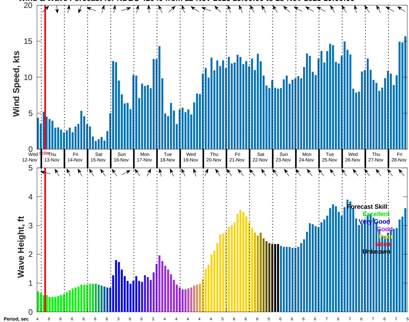
Wind & Wave Forecast for NDBC 42040 from 12-Nov-2025 19:00:00 to 28-Nov-2025 19:00:00
