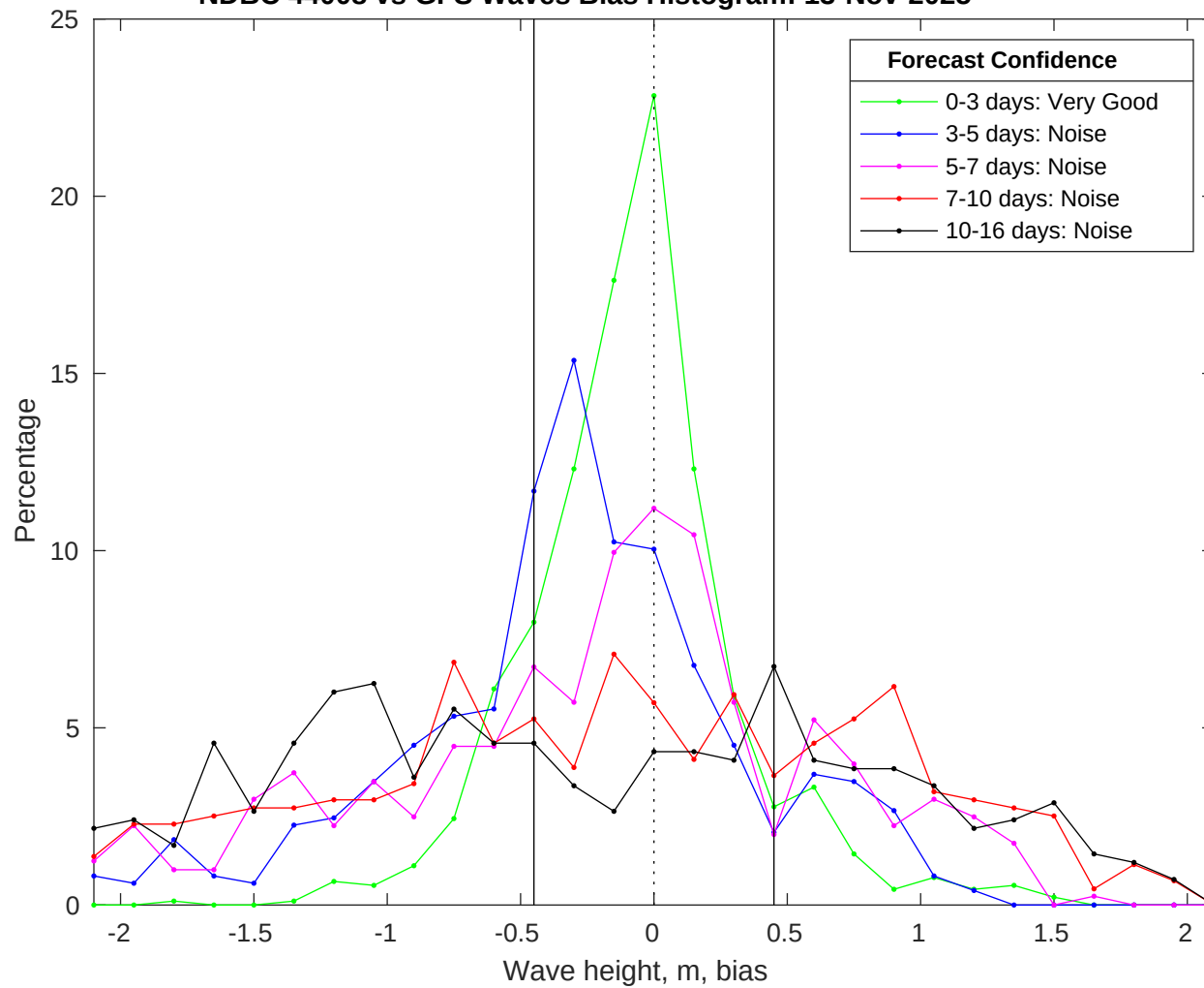
NDBC 44008 vs GFS Waves Bias Histogram: 13-Nov-2025
