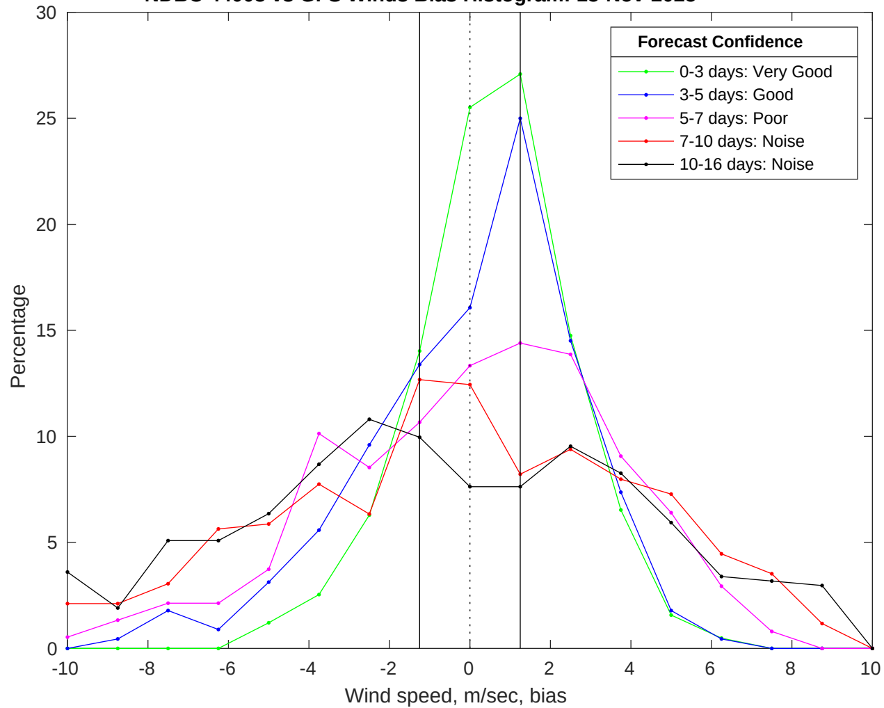
NDBC 44008 vs GFS Winds Bias Histogram: 13-Nov-2025
