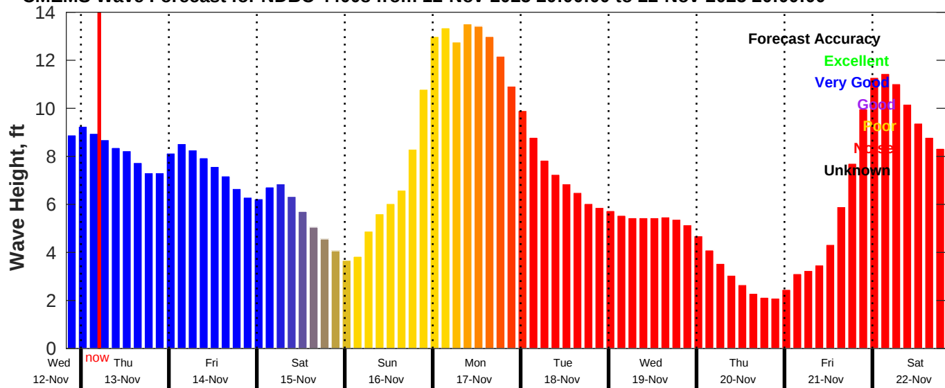
CMEMS Wave Forecast for NDBC 44008 from 12-Nov-2025 20:00:00 to 22-Nov-2025 20:00:00
