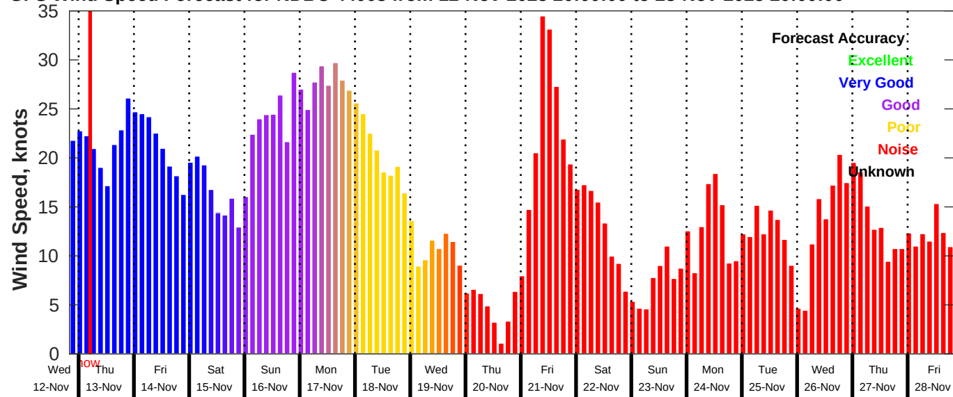
GFS Wind Speed Forecast for NDBC 44008 from 12-Nov-2025 20:00:00 to 28-Nov-2025 20:00:00
