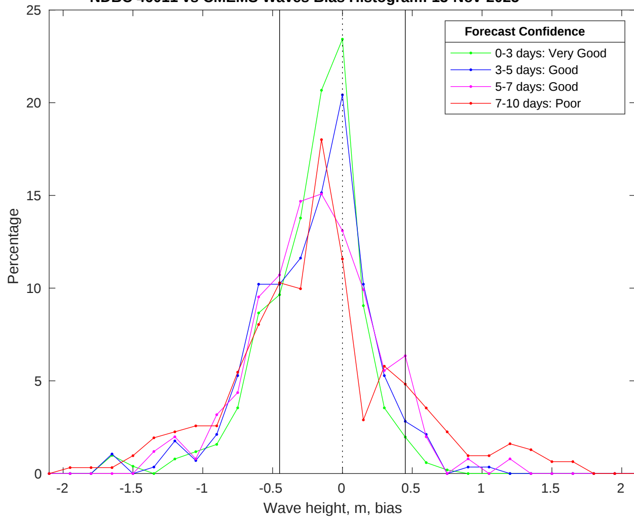
NDBC 46011 vs CMEMS Waves Bias Histogram: 13-Nov-2025
