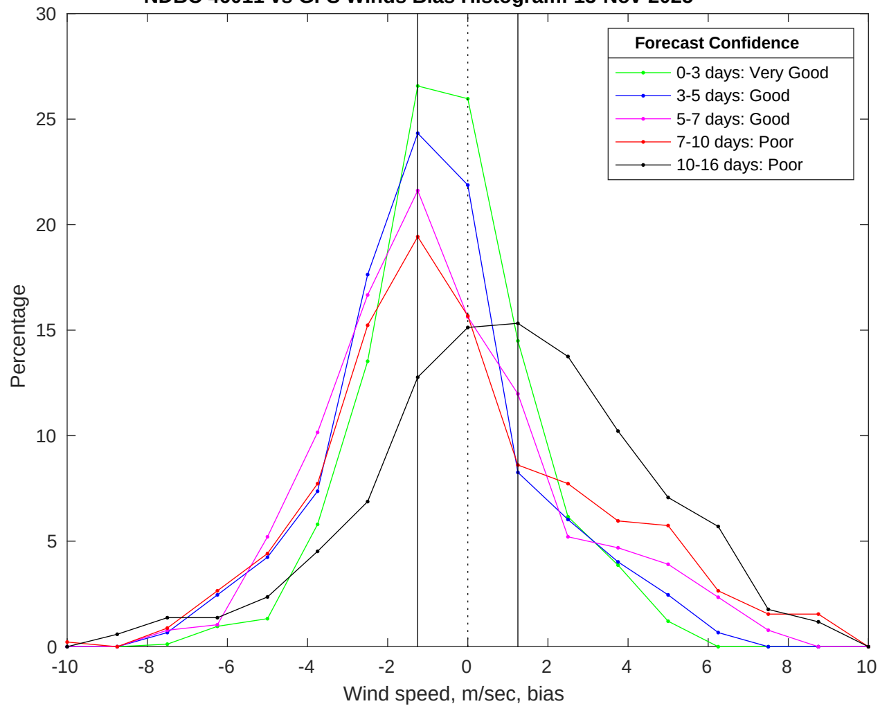
NDBC 46011 vs GFS Winds Bias Histogram: 13-Nov-2025
