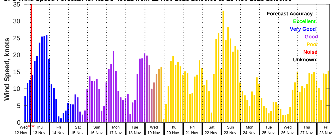
GFS Wind Speed Forecast for NDBC 46011 from 12-Nov-2025 16:00:00 to 28-Nov-2025 16:00:00
