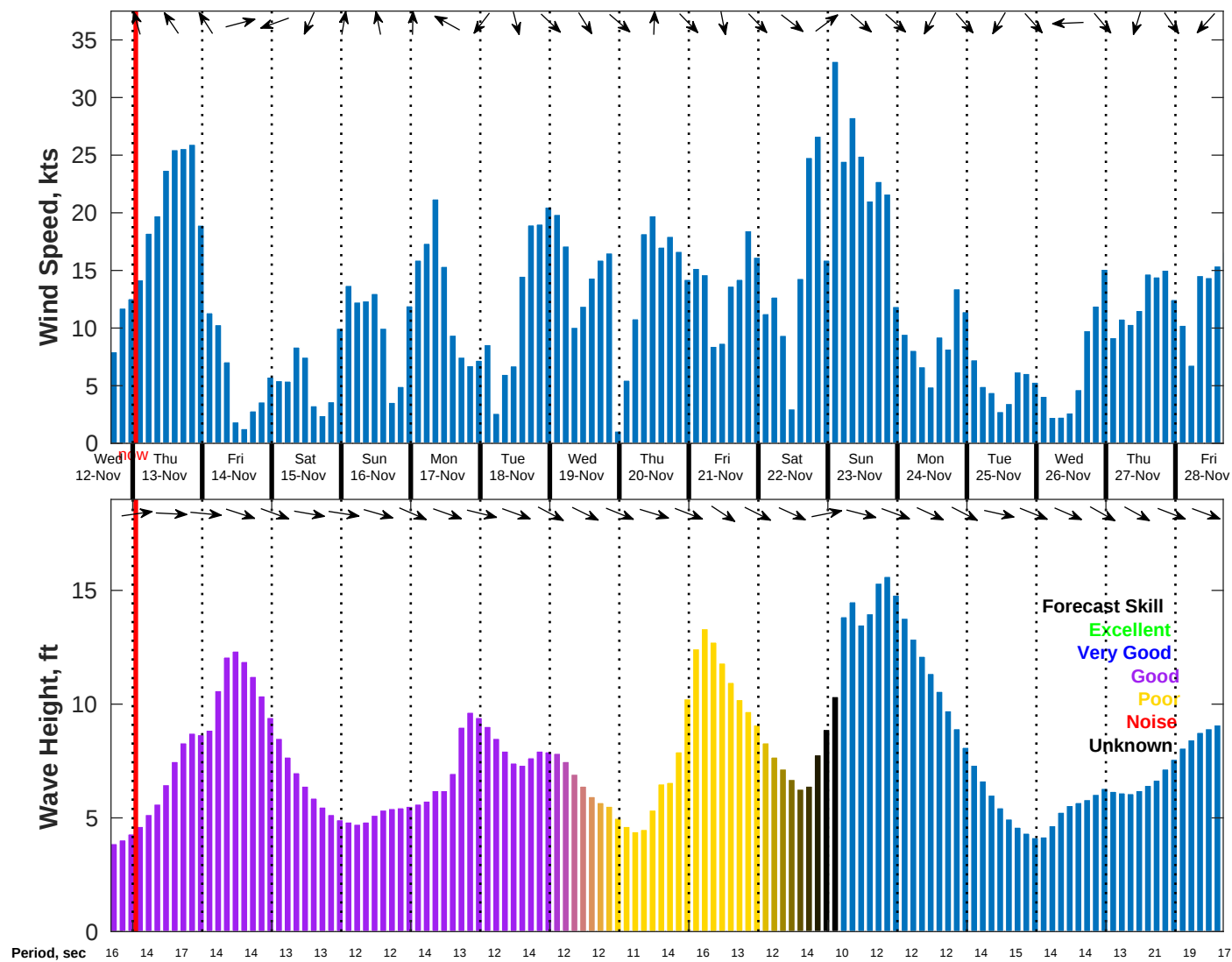
Wind & Wave Forecast for NDBC 46011 from 12-Nov-2025 16:00:00 to 28-Nov-2025 16:00:00
