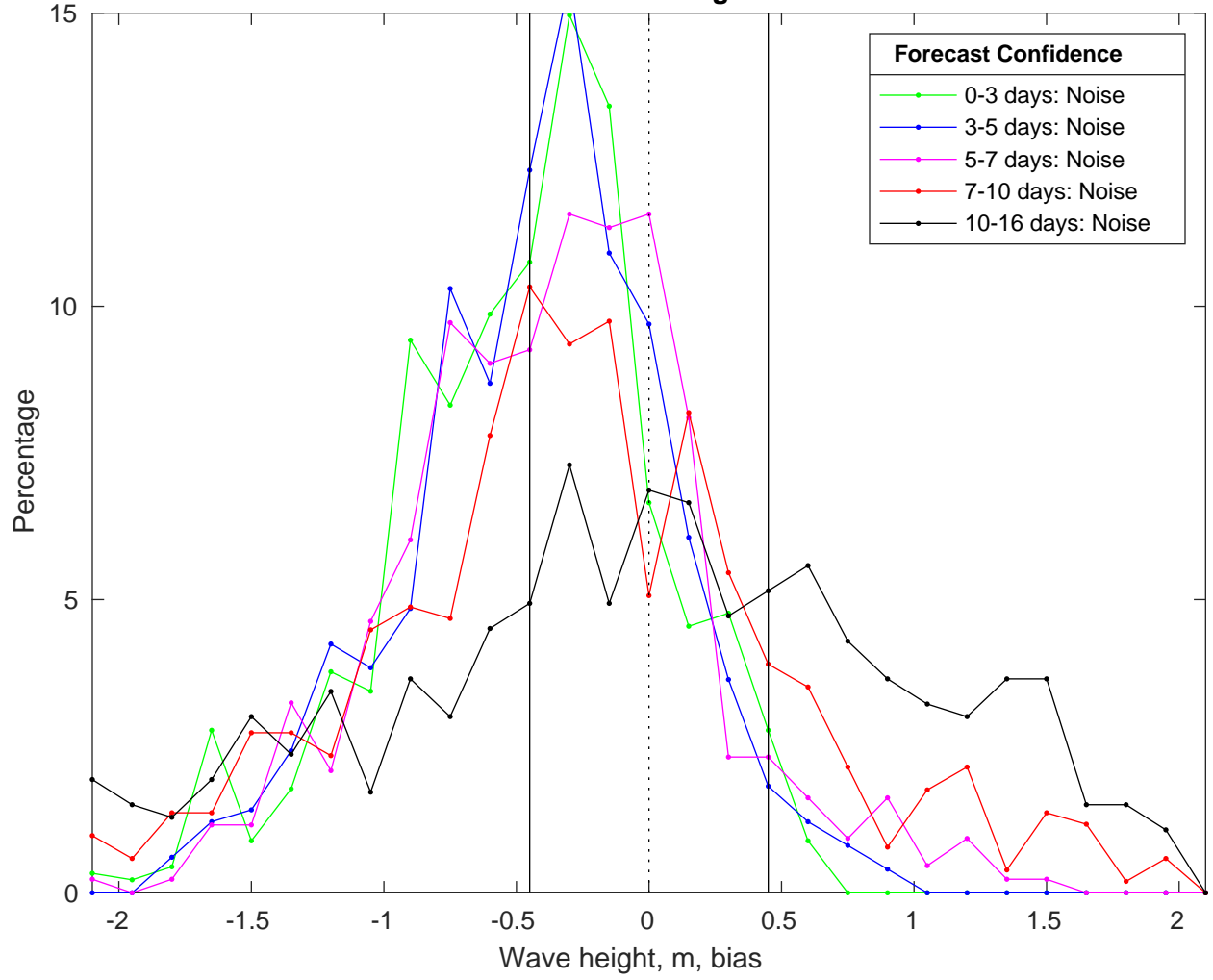
NDBC 46028 vs GFS Waves Bias Histogram: 13-Nov-2025
