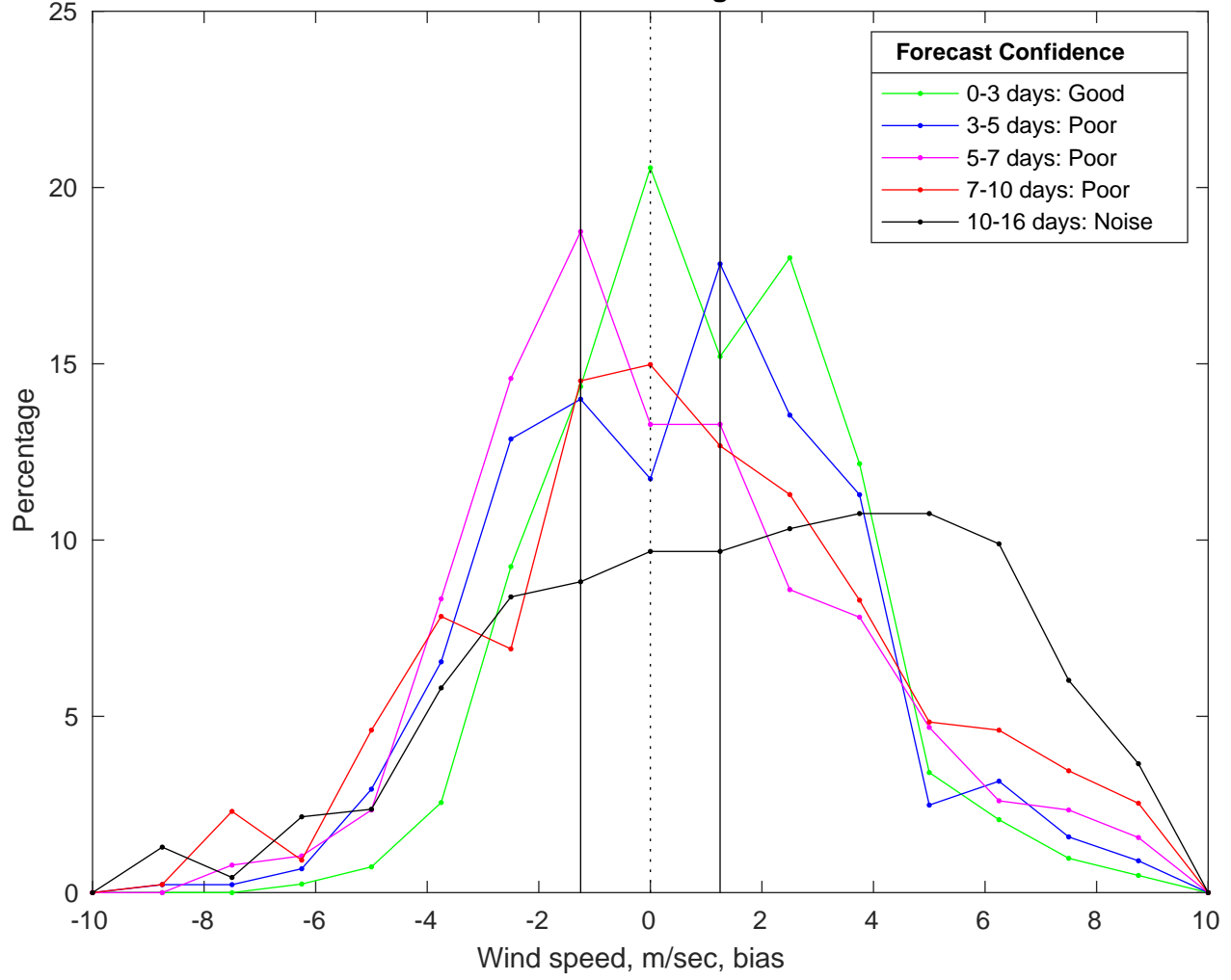
NDBC 46028 vs GFS Winds Bias Histogram: 13-Nov-2025
