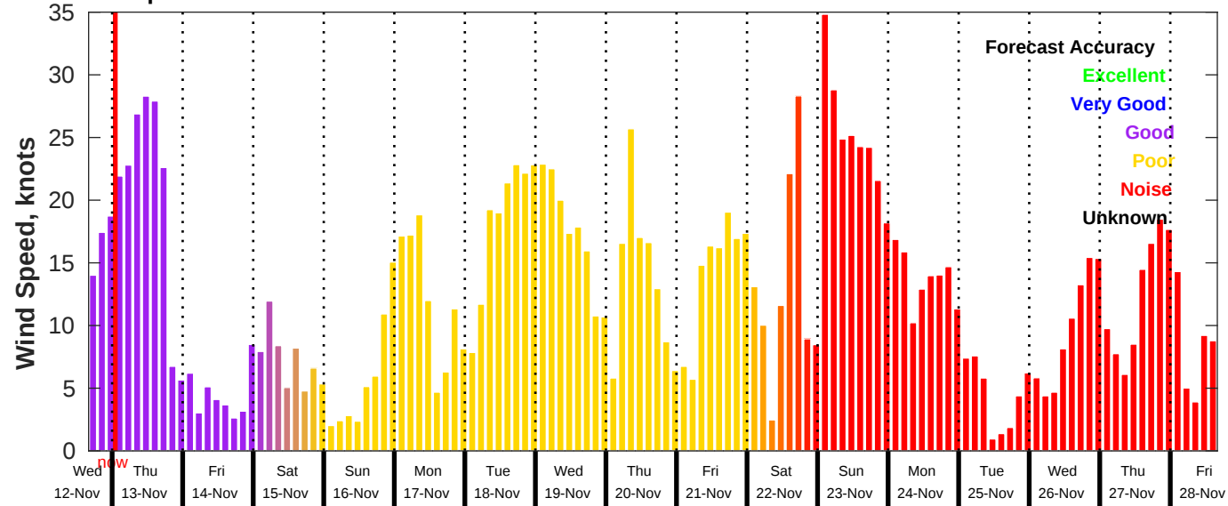
GFS Wind Speed Forecast for NDBC 46028 from 12-Nov-2025 16:00:00 to 28-Nov-2025 16:00:00
