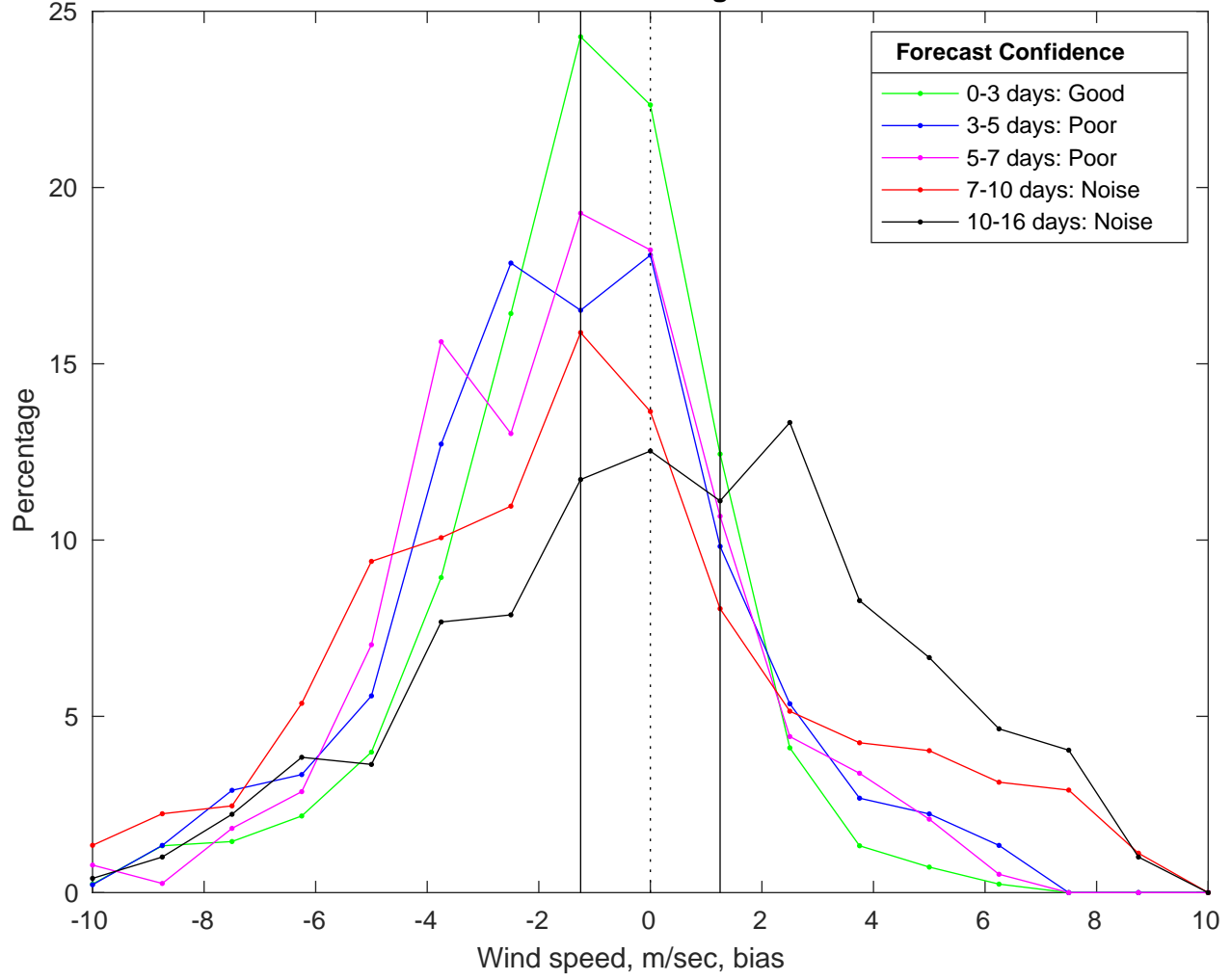
NDBC 46054 vs GFS Winds Bias Histogram: 13-Nov-2025
