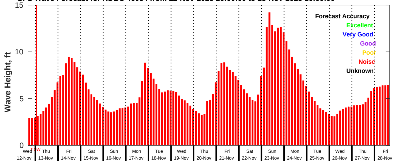
GFS Wave Forecast for NDBC 46054 from 12-Nov-2025 16:00:00 to 28-Nov-2025 16:00:00
