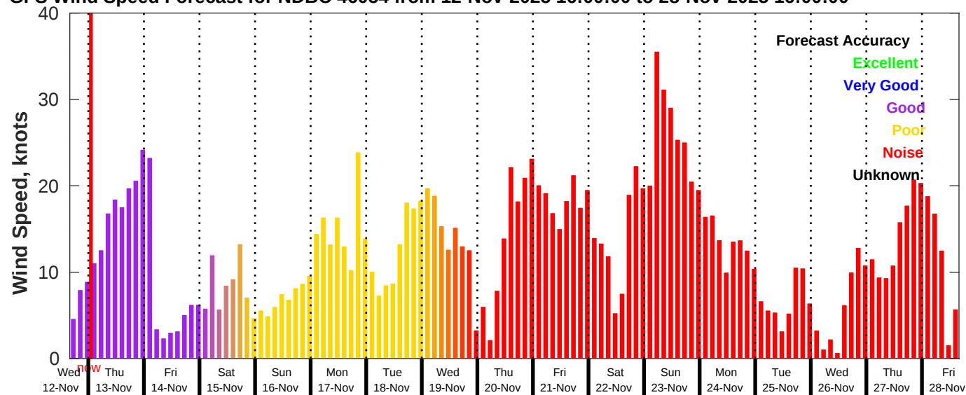
GFS Wind Speed Forecast for NDBC 46054 from 12-Nov-2025 16:00:00 to 28-Nov-2025 16:00:00
