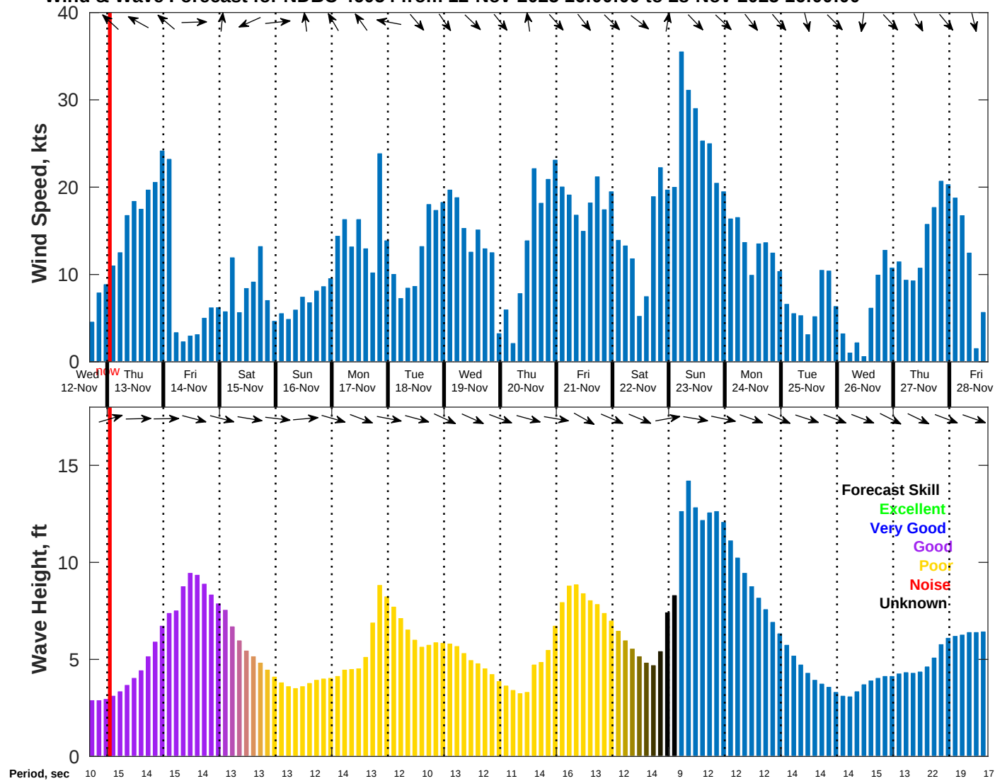
Wind & Wave Forecast for NDBC 46054 from 12-Nov-2025 16:00:00 to 28-Nov-2025 16:00:00
