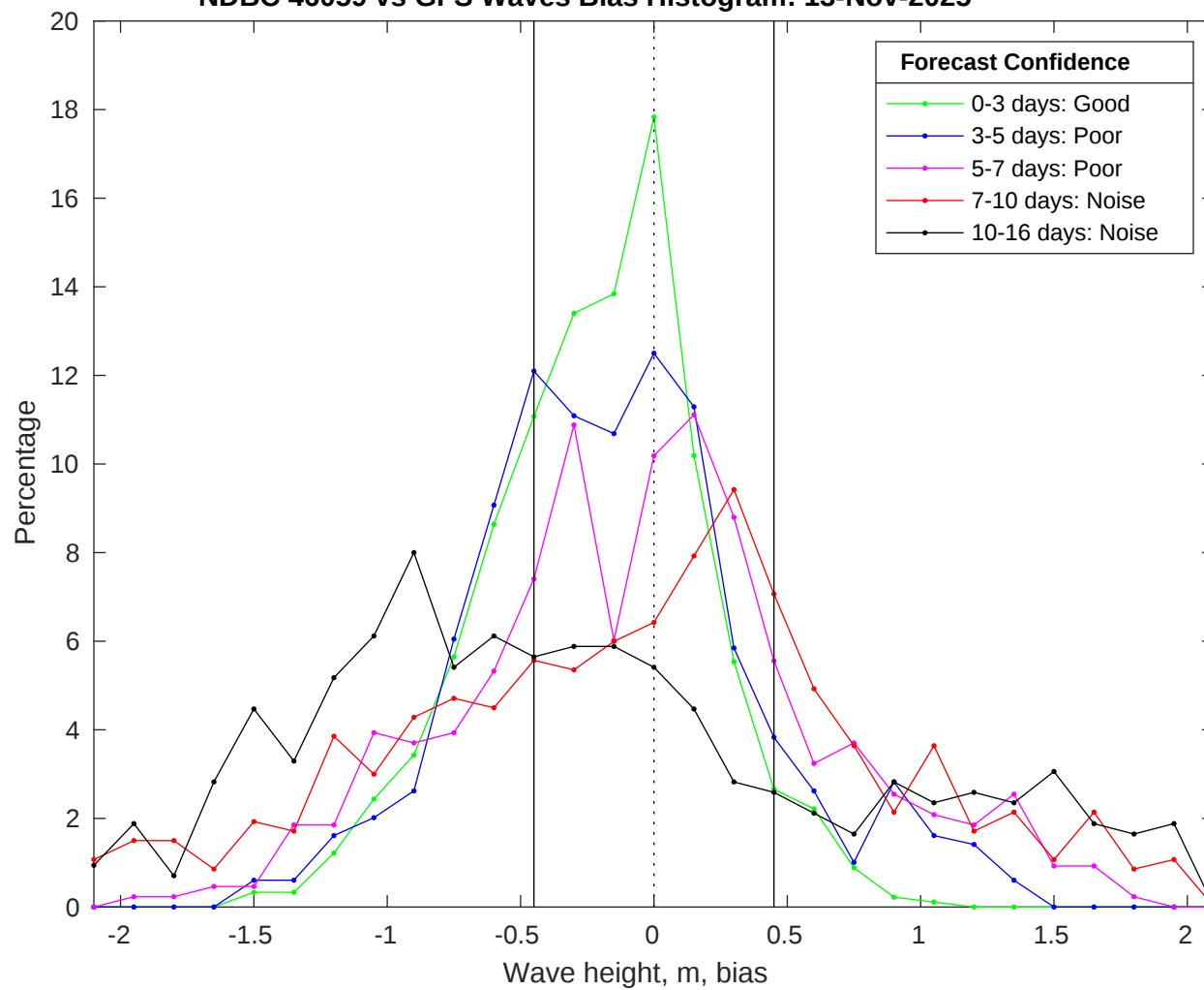
NDBC 46059 vs GFS Waves Bias Histogram: 13-Nov-2025
