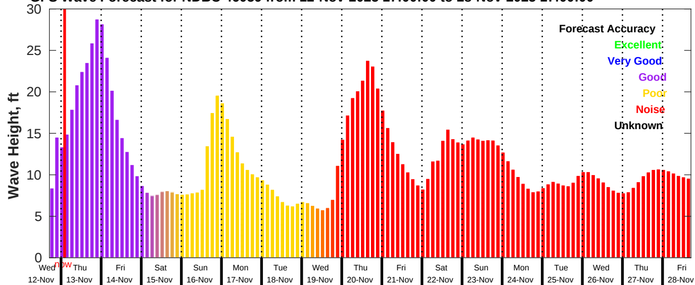
GFS Wave Forecast for NDBC 46059 from 12-Nov-2025 17:00:00 to 28-Nov-2025 17:00:00
