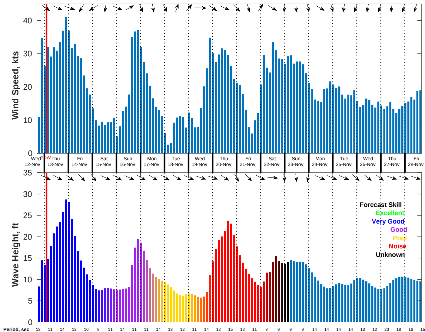
Wind & Wave Forecast for NDBC 46059 from 12-Nov-2025 17:00:00 to 28-Nov-2025 17:00:00
