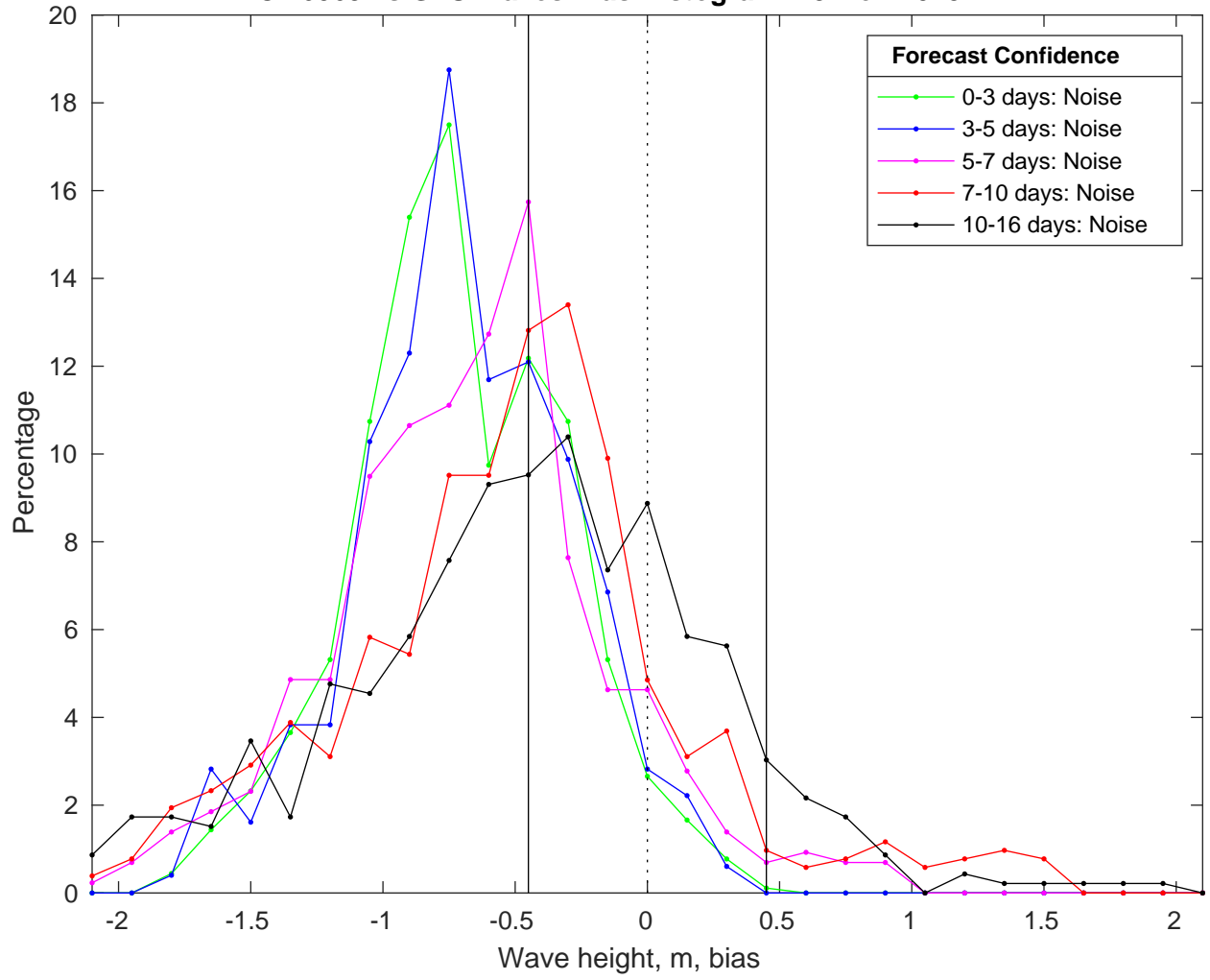
NDBC 46069 vs GFS Waves Bias Histogram: 13-Nov-2025
