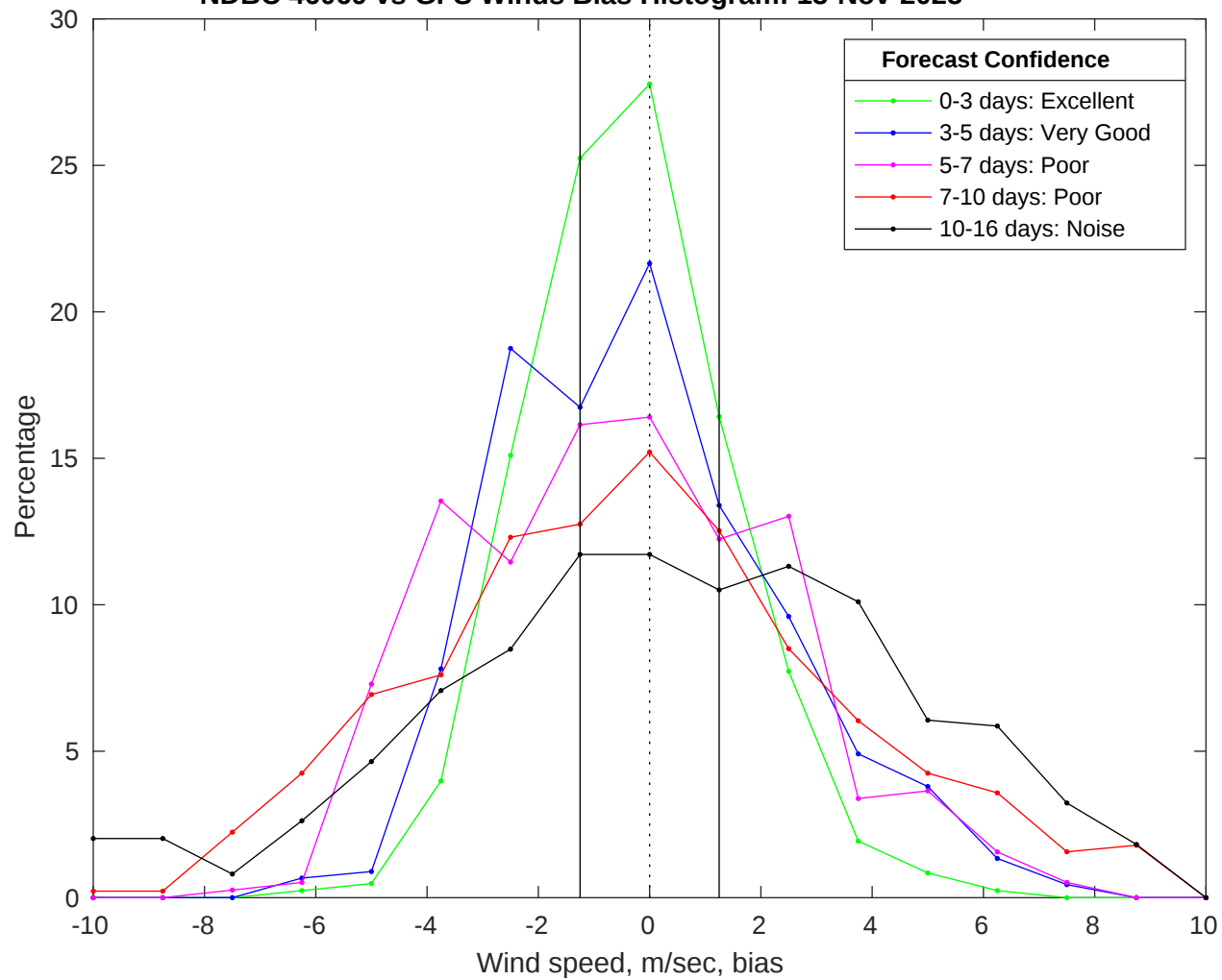
NDBC 46069 vs GFS Winds Bias Histogram: 13-Nov-2025
