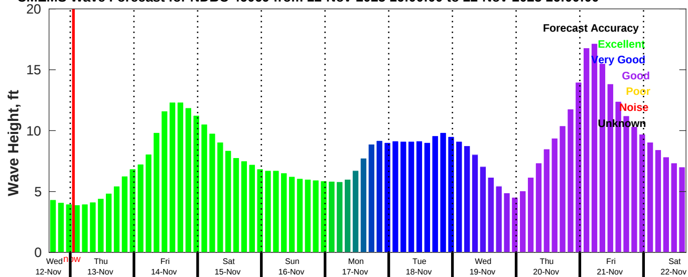
CMEMS Wave Forecast for NDBC 46069 from 12-Nov-2025 16:00:00 to 22-Nov-2025 16:00:00
