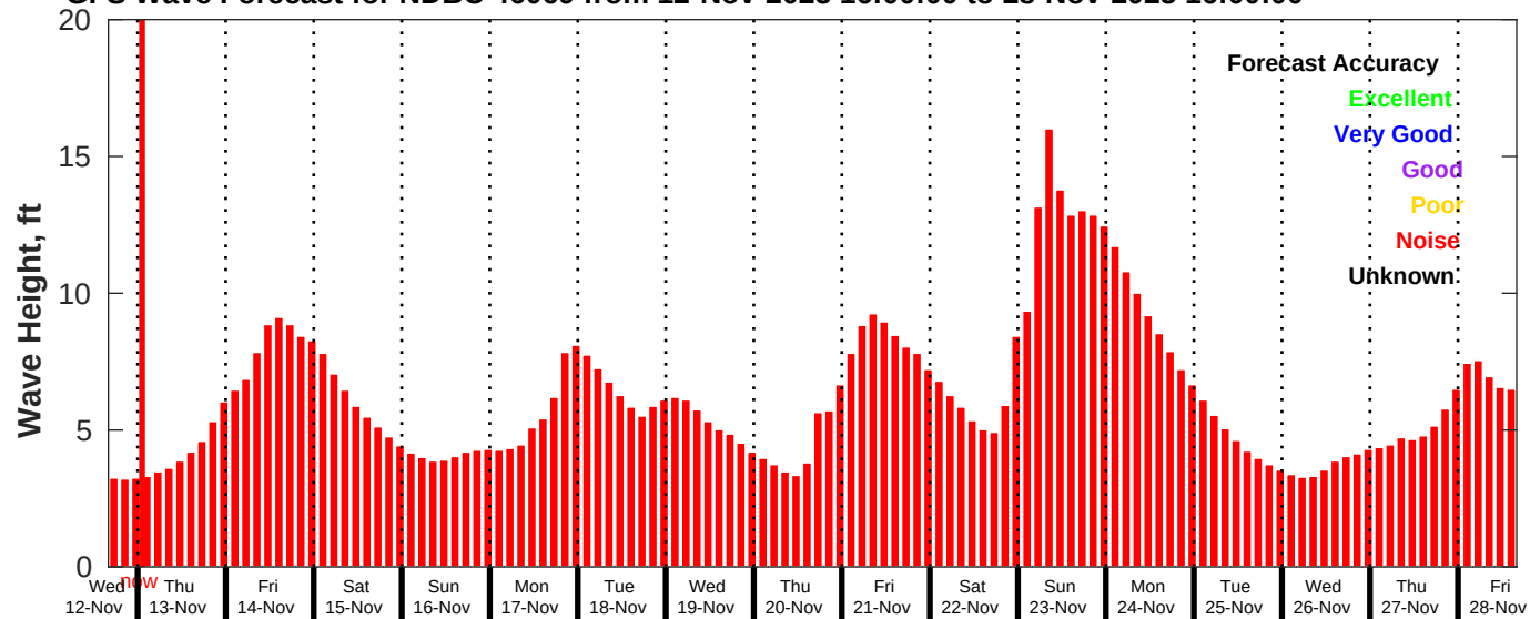
GFS Wave Forecast for NDBC 46069 from 12-Nov-2025 16:00:00 to 28-Nov-2025 16:00:00
