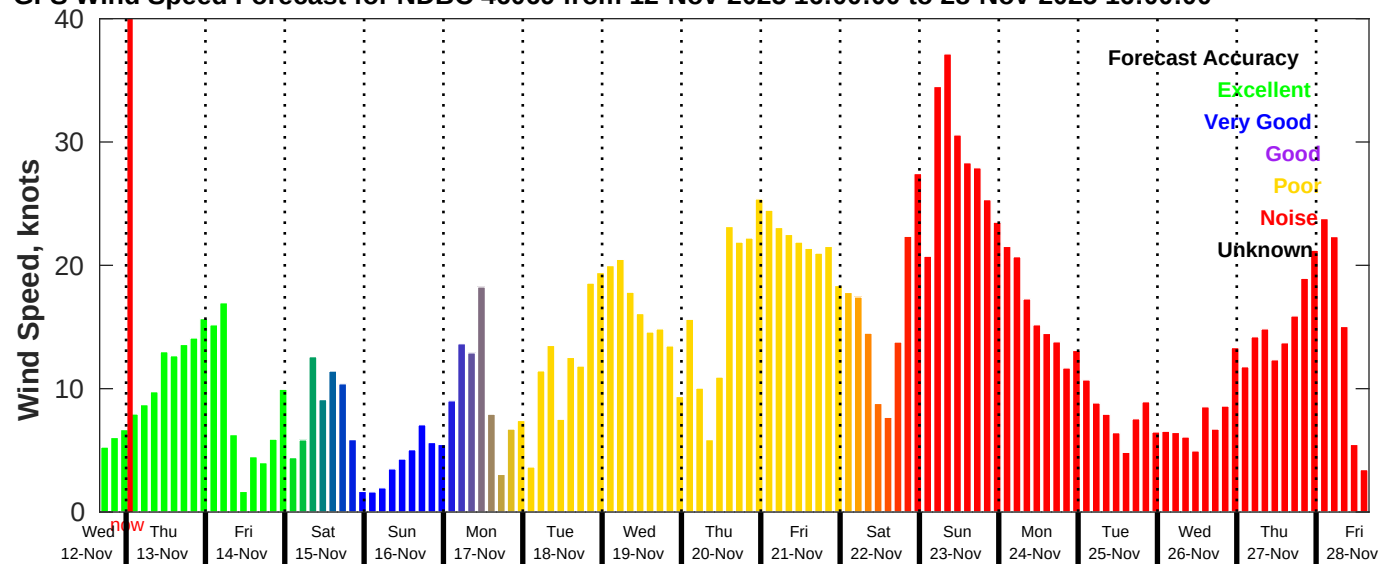
GFS Wind Speed Forecast for NDBC 46069 from 12-Nov-2025 16:00:00 to 28-Nov-2025 16:00:00
