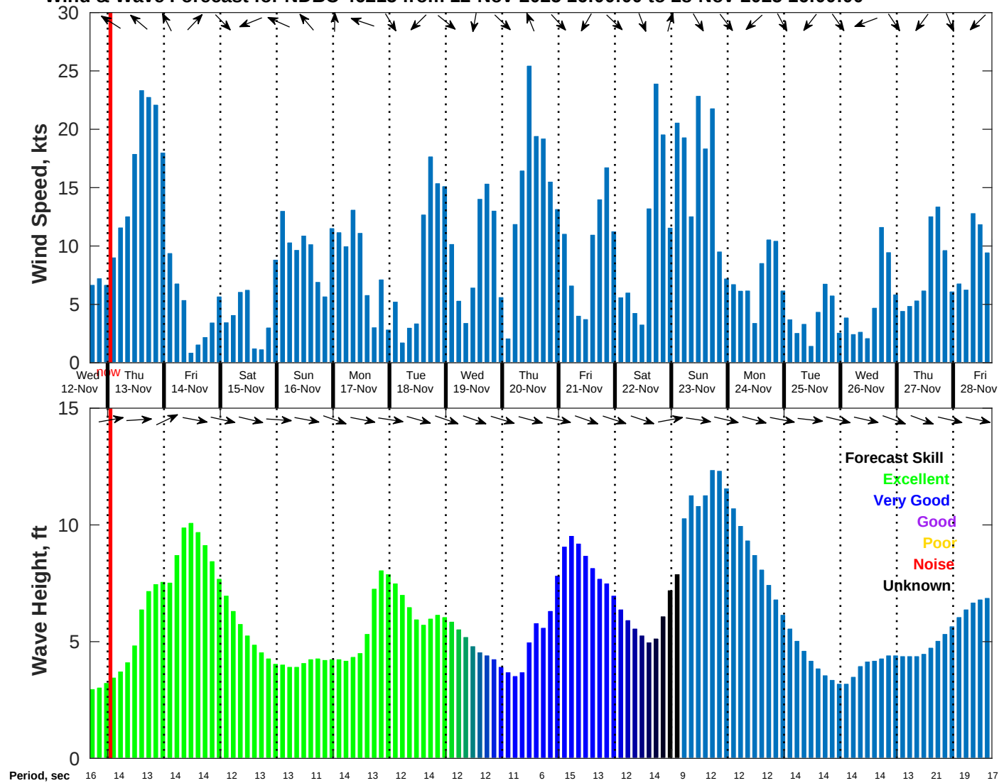
Wind & Wave Forecast for NDBC 46215 from 12-Nov-2025 16:00:00 to 28-Nov-2025 16:00:00
