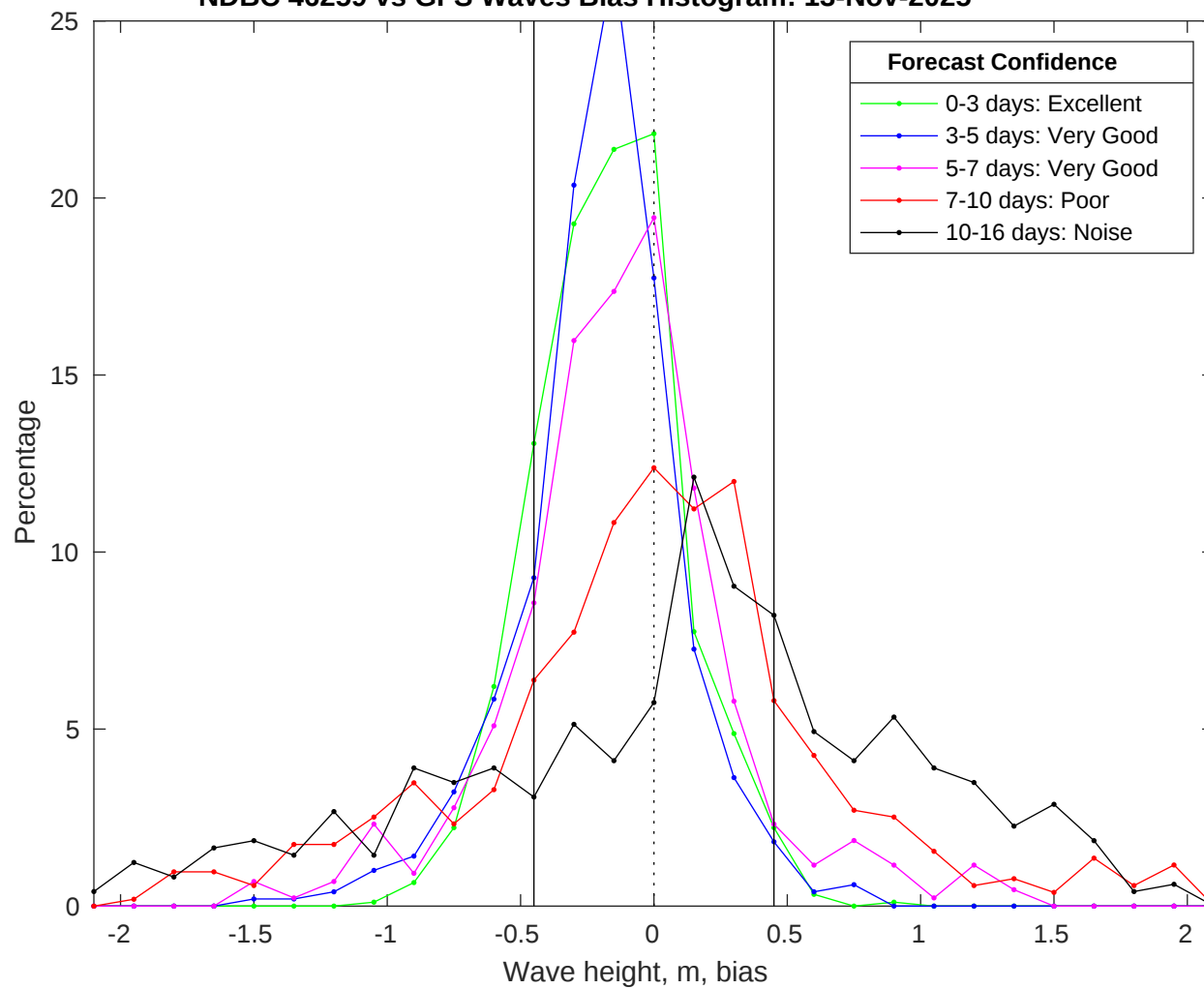
NDBC 46259 vs GFS Waves Bias Histogram: 13-Nov-2025
