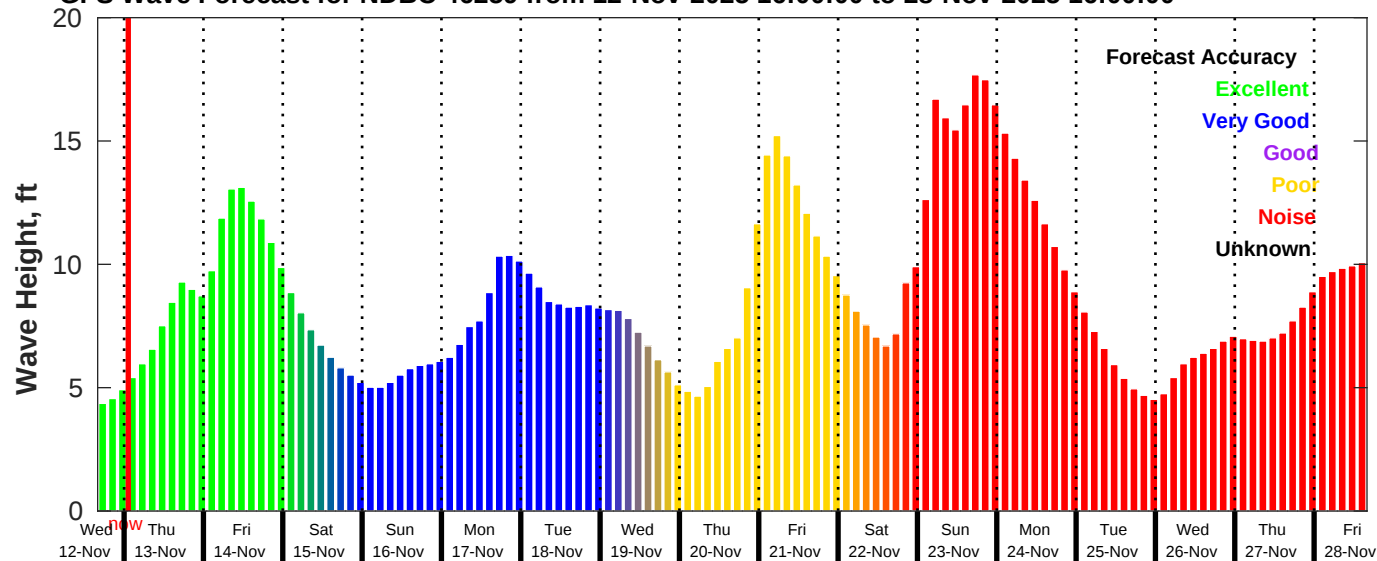
GFS Wave Forecast for NDBC 46259 from 12-Nov-2025 16:00:00 to 28-Nov-2025 16:00:00
