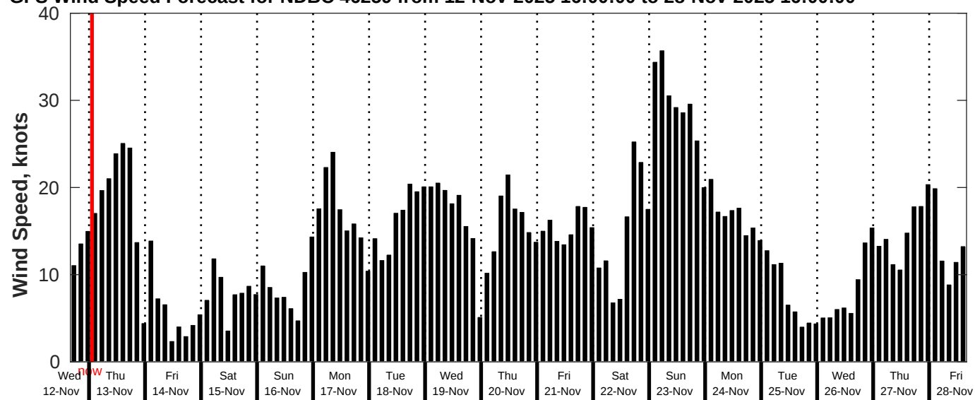
GFS Wind Speed Forecast for NDBC 46259 from 12-Nov-2025 16:00:00 to 28-Nov-2025 16:00:00
