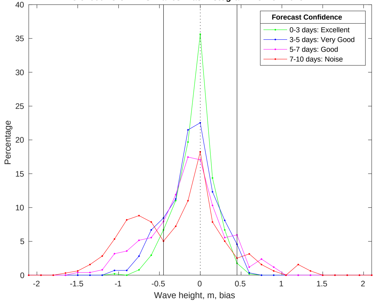
NDBC 51000 vs CMEMS Waves Bias Histogram: 13-Nov-2025
