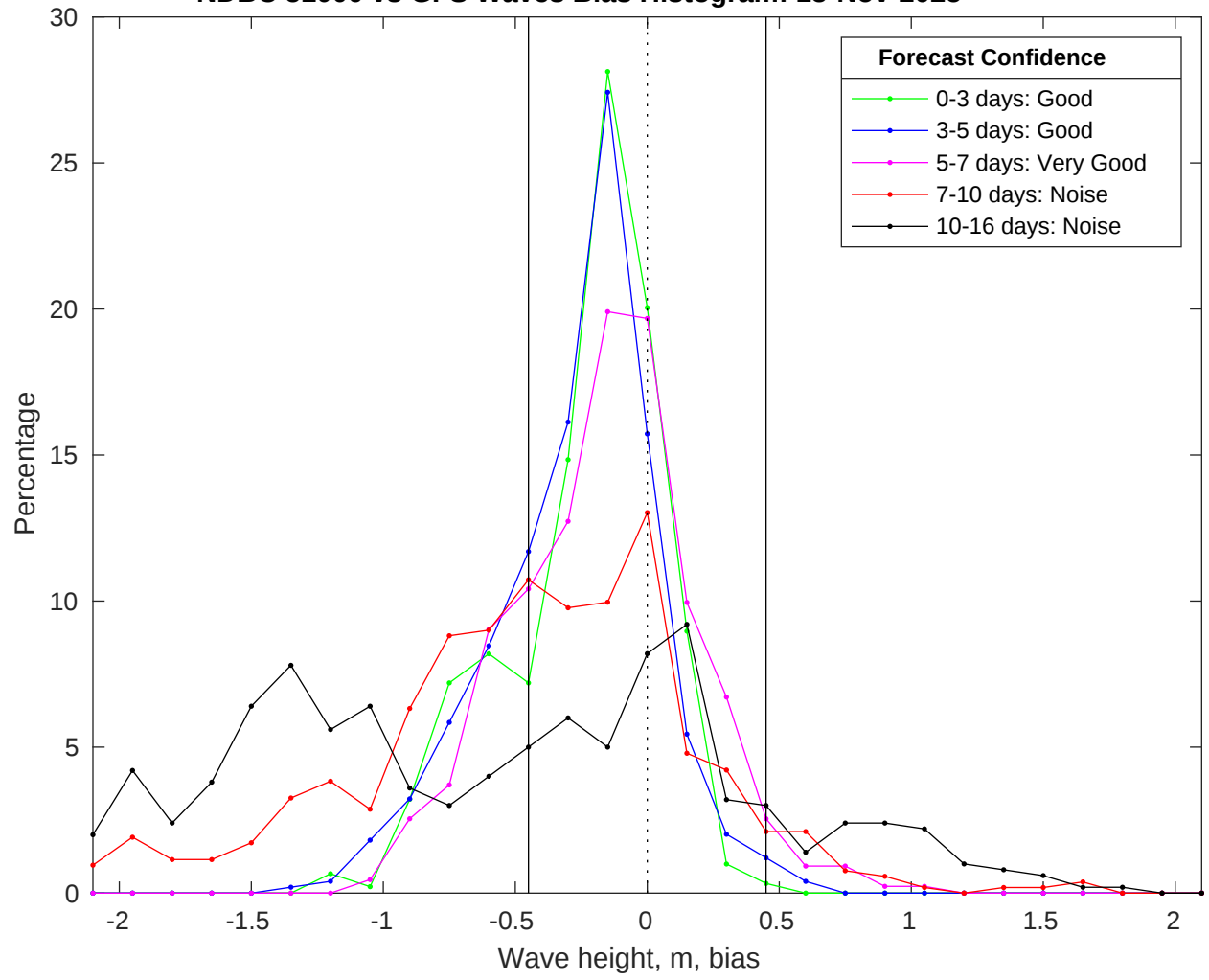
NDBC 51000 vs GFS Waves Bias Histogram: 13-Nov-2025
