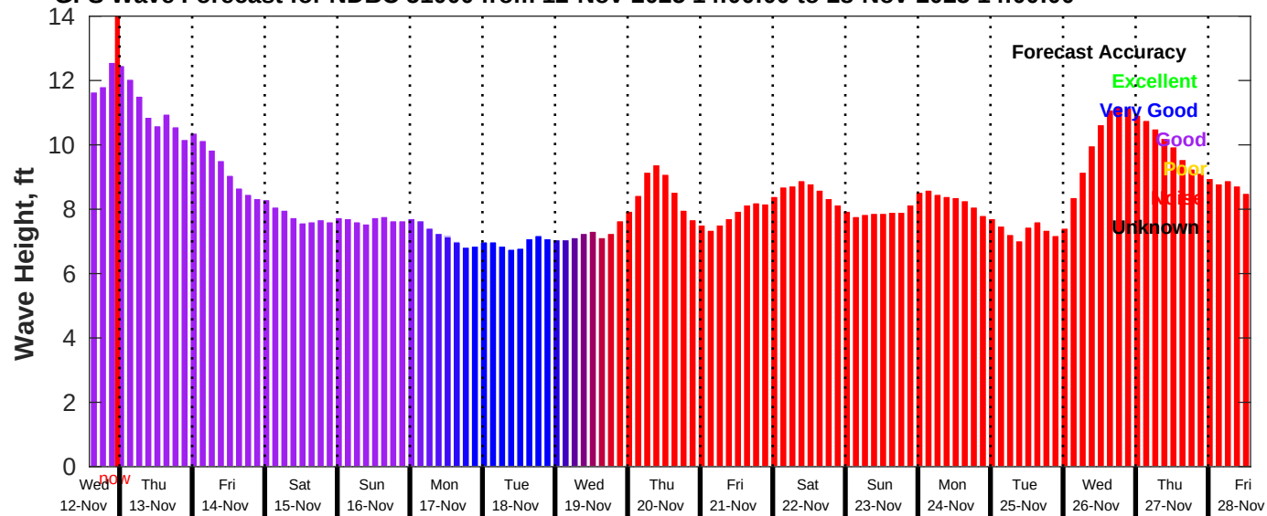
GFS Wave Forecast for NDBC 51000 from 12-Nov-2025 14:00:00 to 28-Nov-2025 14:00:00
