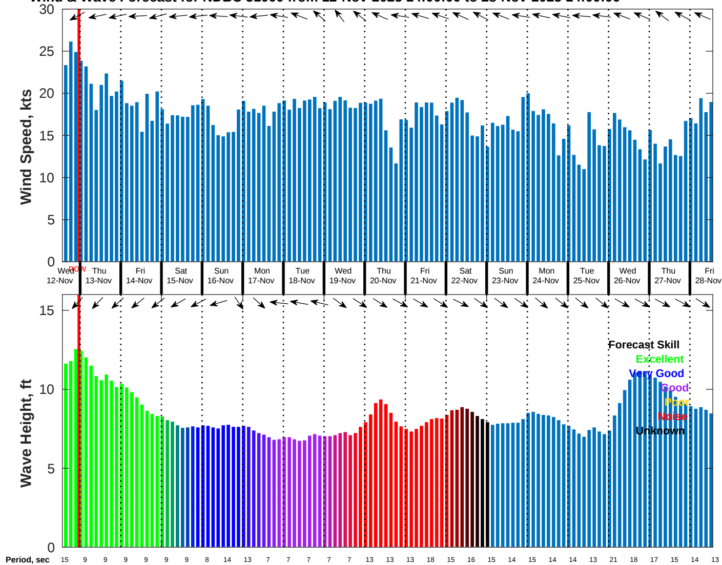
Wind & Wave Forecast for NDBC 51000 from 12-Nov-2025 14:00:00 to 28-Nov-2025 14:00:00
