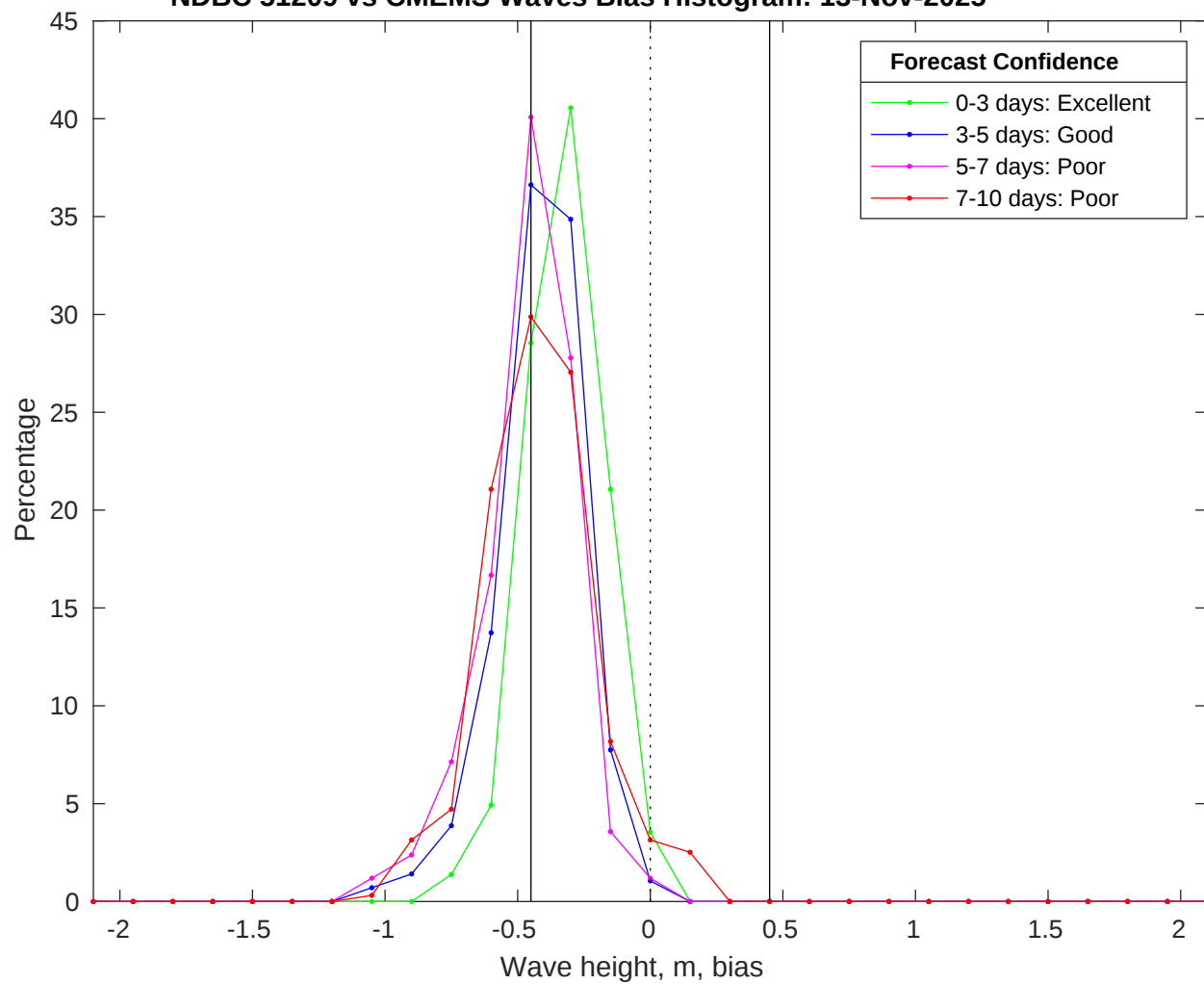
NDBC 51209 vs CMEMS Waves Bias Histogram: 13-Nov-2025
