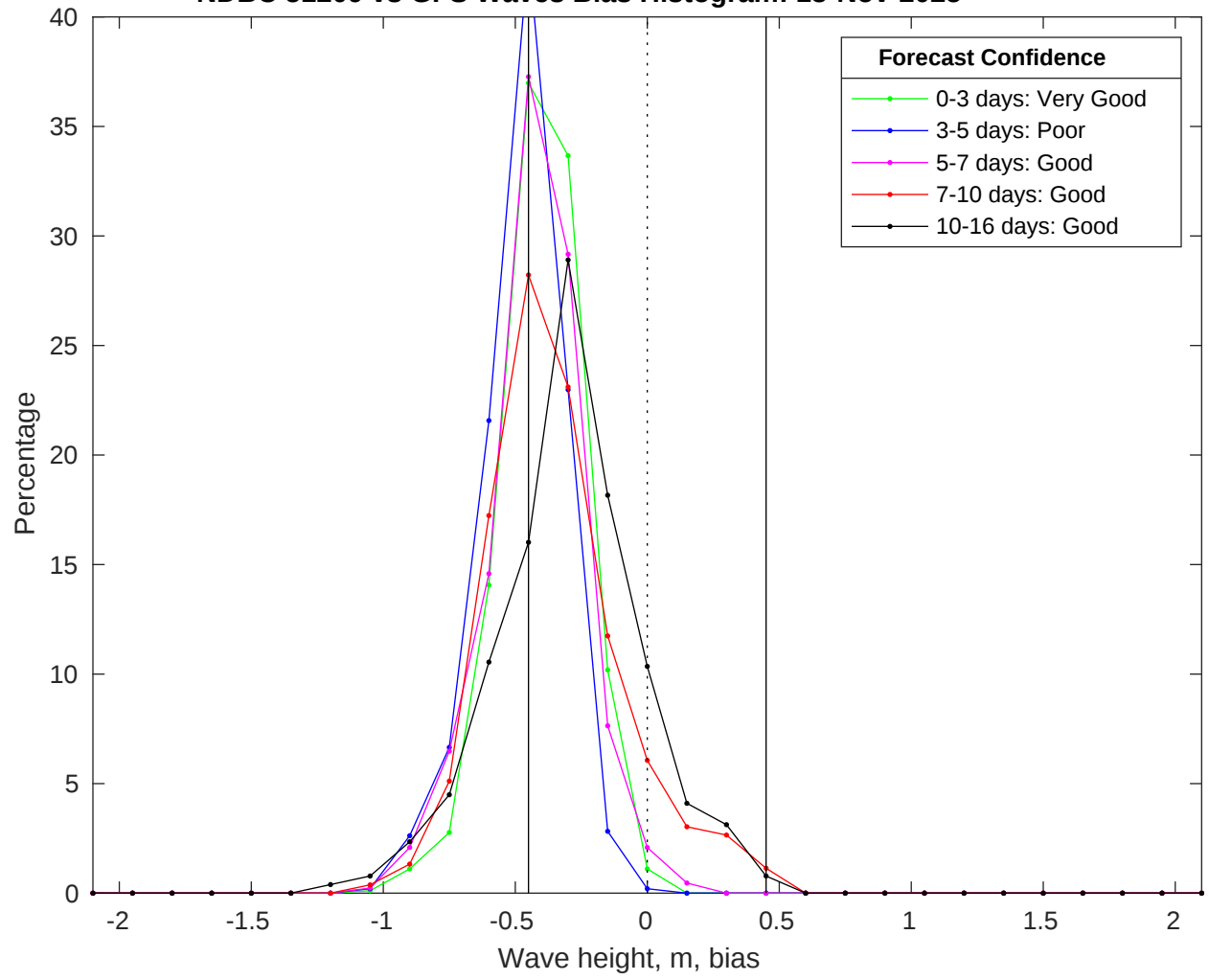
NDBC 51209 vs GFS Waves Bias Histogram: 13-Nov-2025
