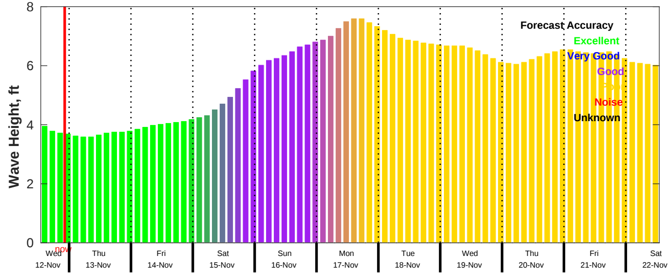
CMEMS Wave Forecast for NDBC 51209 from 12-Nov-2025 13:00:00 to 22-Nov-2025 13:00:00
