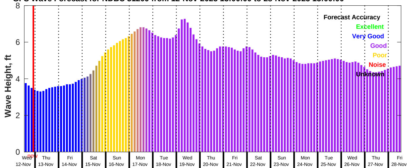
GFS Wave Forecast for NDBC 51209 from 12-Nov-2025 13:00:00 to 28-Nov-2025 13:00:00
