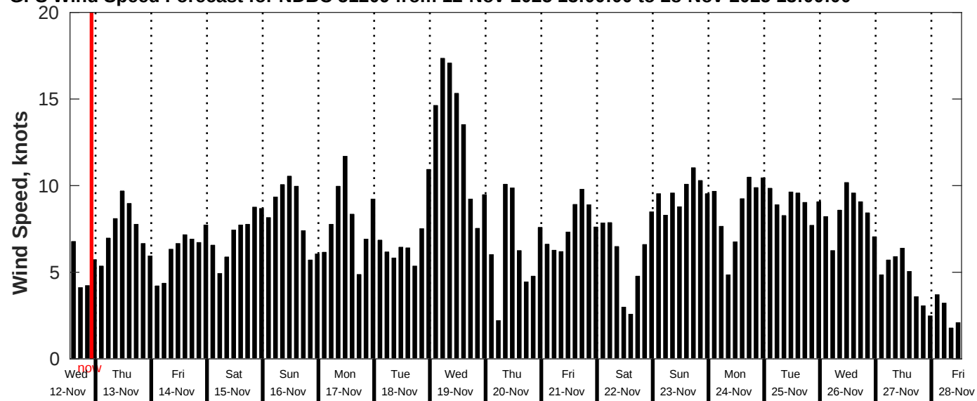
GFS Wind Speed Forecast for NDBC 51209 from 12-Nov-2025 13:00:00 to 28-Nov-2025 13:00:00
